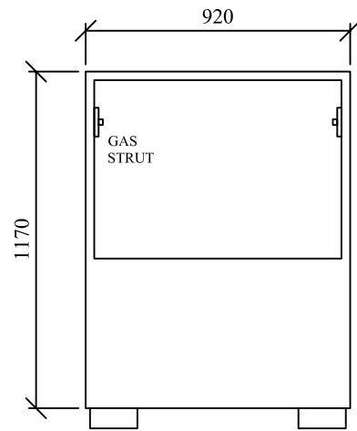
VIEW OF ACCESS OPENING - LID REMOVED
