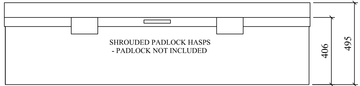
TRUCK BOX WITH LID CLOSED
