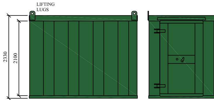
FLAT ROOF PAINTED PROFILE STEEL OUTER FINISH
