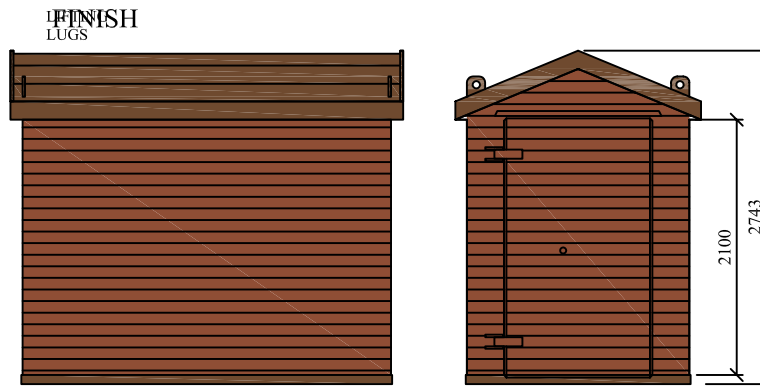
TILE EFFECT ROOF TIMBER CLAD OUTER FINISH
