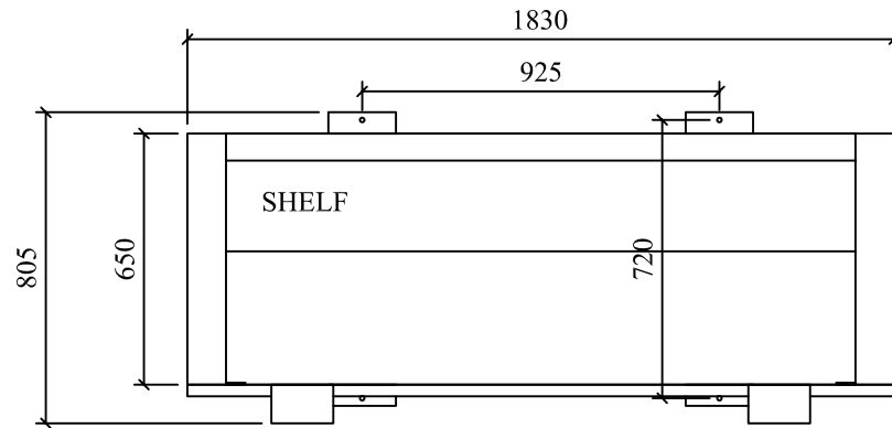
PLAN - CLOSED, LID REMOVED
