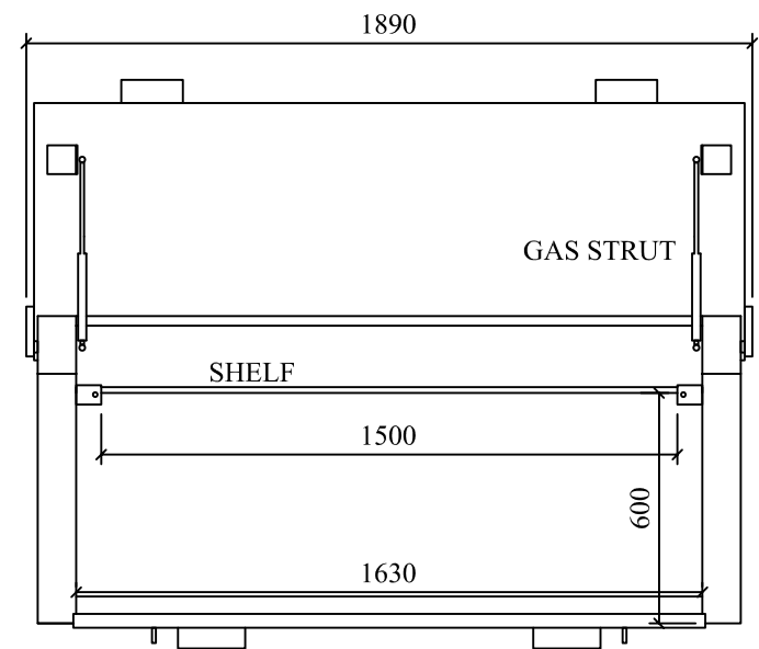
FRONT ELEVATION - OPEN
