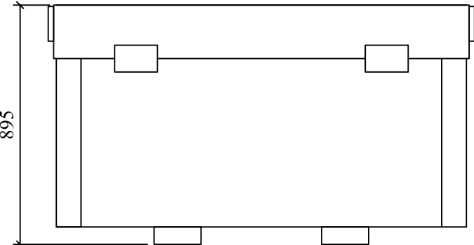
FRONT ELEVATION - CLOSED
