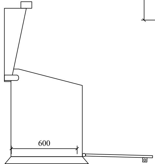
SIDE ELEVATION - LID UP AND FRONT DOWN
