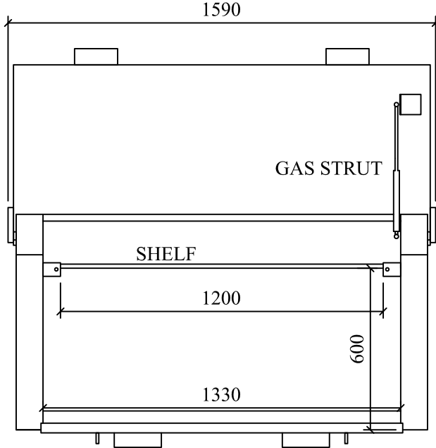
FRONT ELEVATION - OPEN
