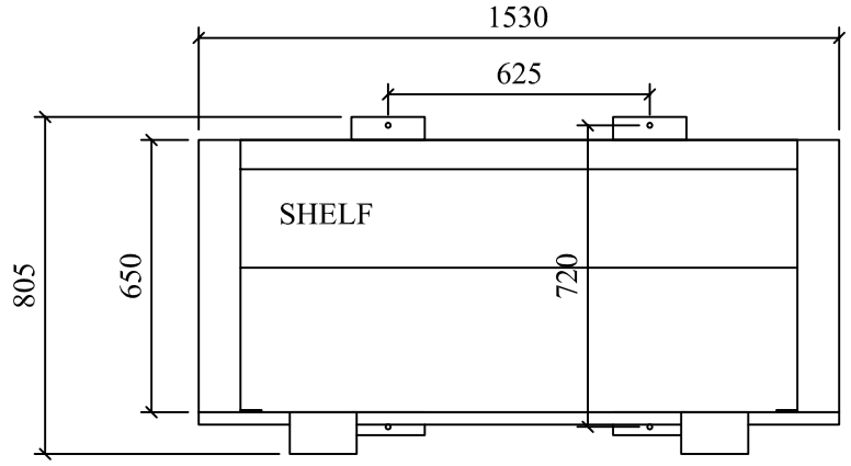
PLAN - CLOSED, LID REMOVED
