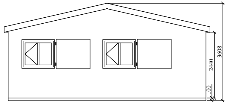
SIDE ELEVATION
