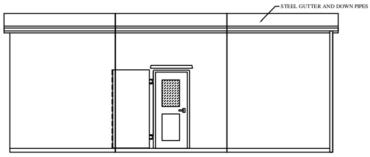
FRONT ELEVATION
