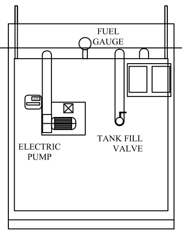
SECTION
