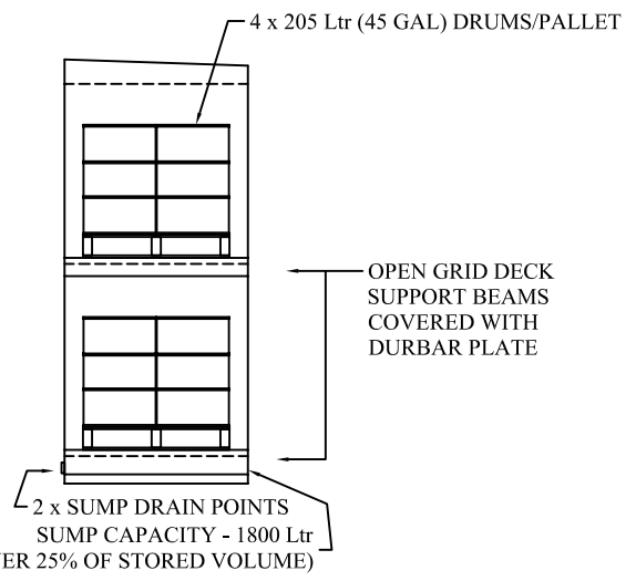
TYPICAL SECTION
