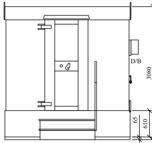
SIDE ELEVATION
