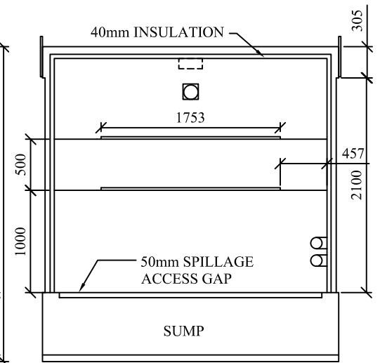
SECTION
