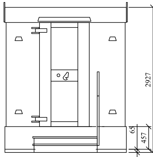
FRONT ELEVATION
