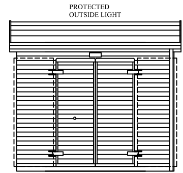
FRONT ELEVATION
