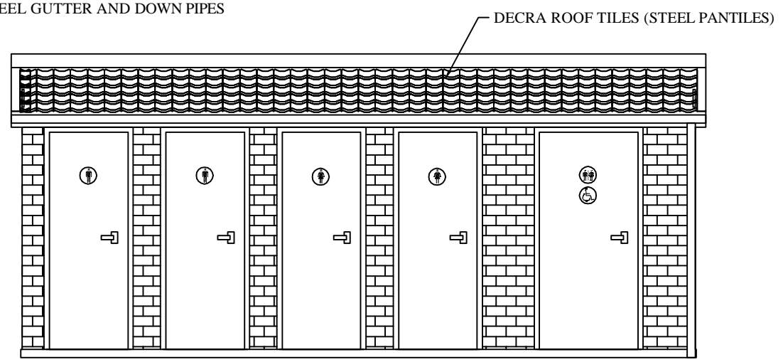
FRONT ELEVATION
