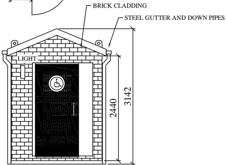
FRONT ELEVATION
